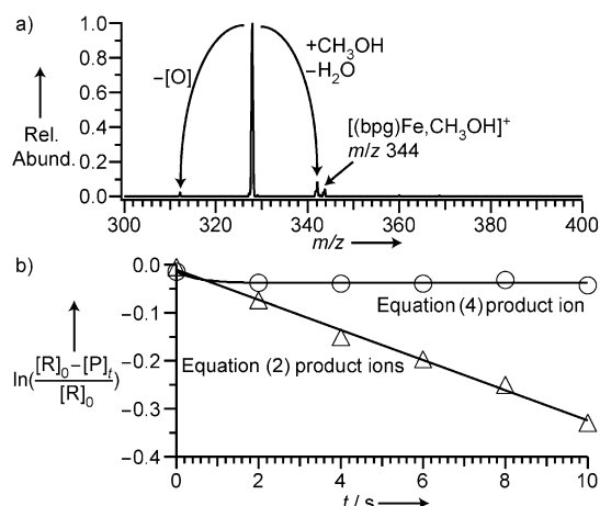
Figure 3. a) Mass spectrum obtained upon storing isolated [(\text{bpg})\text{FeO}]^+ for 2 s in the presence of methanol ( 0.6 \times 10^{-6} Torr), and b) kinetic plot (see Supporting Information for details) for the O-atom transfer reaction pathway [Eq. (2)] and addition/elimination reaction pathway [Eq. (4)].
