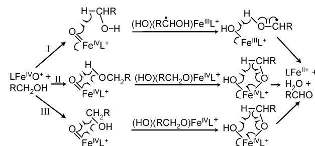
Scheme 1. Possible mechanisms for primary alcohol oxidation by a \text{Fe}^{\text{IV}}\text{O} complex ion, where L is a ligand.
